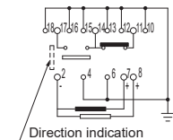
2 coil latching type (Reset condition)
