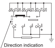
Single side stable type (Deenergized condition)
