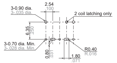
PC board pattern (Bottom view)
