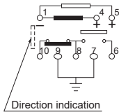
2 coil latching type (Reset condition)
