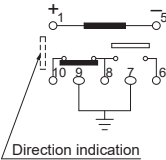
1 coil latching type (Reset condition)
