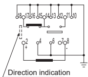
1 coil latching type (Reset condition)
