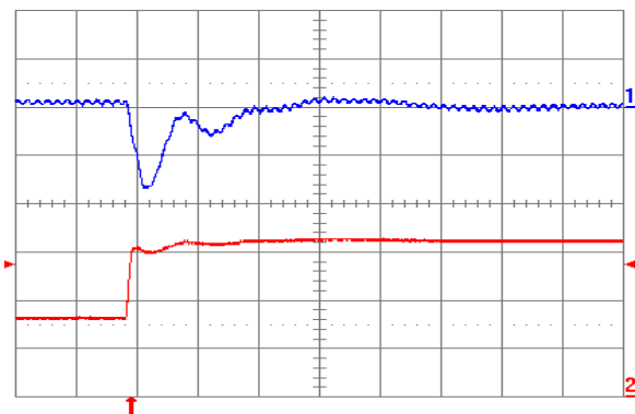
Fig. 2.0V.6: Output voltage response for V_{out} = 2.0\text{ V} to positive load current step change from 8 A to 16 A with slew rate of 5\text{ A}/\mu\text{s} at V_{in} = 5\text{ V} . Top trace: output voltage (100 mV/div.); Bottom trace: load current (5 A/div.). C_o = 100\text{ }\mu\text{F} ceramic + 1\text{ }\mu\text{F} ceramic. Time scale: 20 \mu\text{s} /div.
