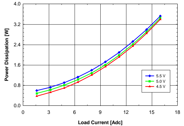
Fig. 3.3V.3: Power loss vs. load current and input voltage for V_{out} = 3.3\text{ V} converter mounted vertically with air flowing from pin 10 to pin 1 at a rate of 200 LFM (1 m/s) and T_a = 25\text{ }^{\circ}\text{C} .
