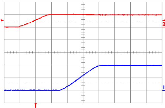
Fig. 2.0V.4: Turn-on transient for V_{out} = 2.0\text{ V} with application of V_{in} at full rated load current (resistive) and 100\text{ }\mu\text{F} external capacitance at V_{in} = 5\text{ V} . Top trace: V_{in} (5 V/div.); Bottom trace: output voltage (1 V/div.); Time scale: 2 ms/div.
