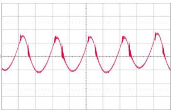
Figure 38. Input reflected ripple current, i_c (500 mA/div.), measured at input terminals at full rated load current and V_{in} = 48 V. Refer to Fig. 37 for test setup. Time scale: 2 \mu s/div.
