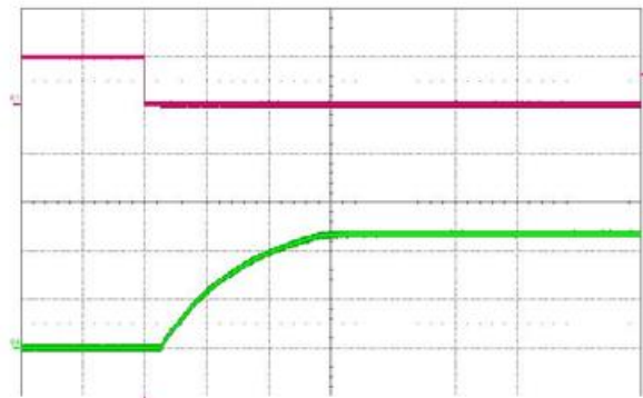
Figure 33. Turn-on transient at full rated load current (resistive) plus 20,000 \mu\text{F} at V_{in} = 48\text{V} , triggered via ON/OFF pin. Top trace: ON/OFF signal (5 V/div.). Bottom trace: output voltage (5 V/div.). Time scale: 5 ms/div
