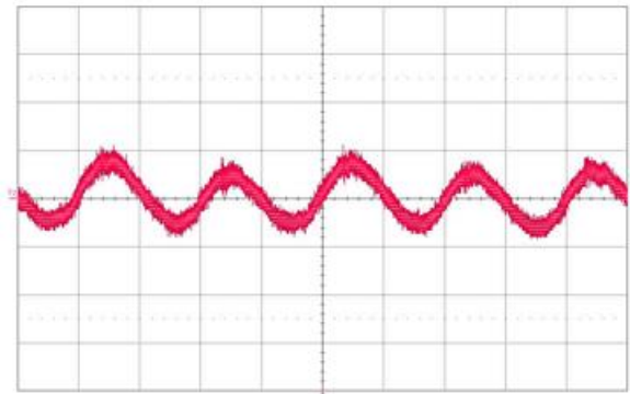
Figure 39. Input reflected ripple current, i_s (50 mA/div.), measured through 5 \mu H at the source at full rated load current and V_{in} = 48 V. Refer to Fig. 37 for test setup. Time scale: 2 \mu s/div.
