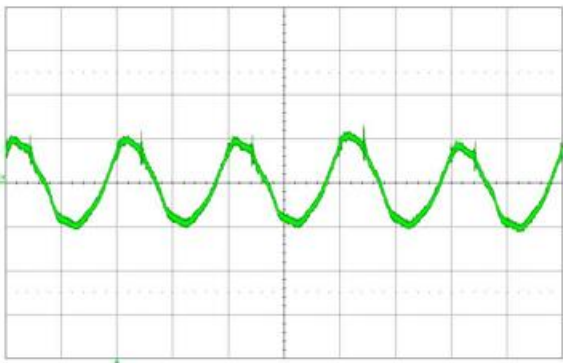
Figure 36. Output voltage ripple (20 mV/div.) at full rated load current into a resistive load with C_o = 10 \mu F tantalum + 1 \mu F ceramic and V_{in} = 48 V. Time scale: 2 \mu s/div.
