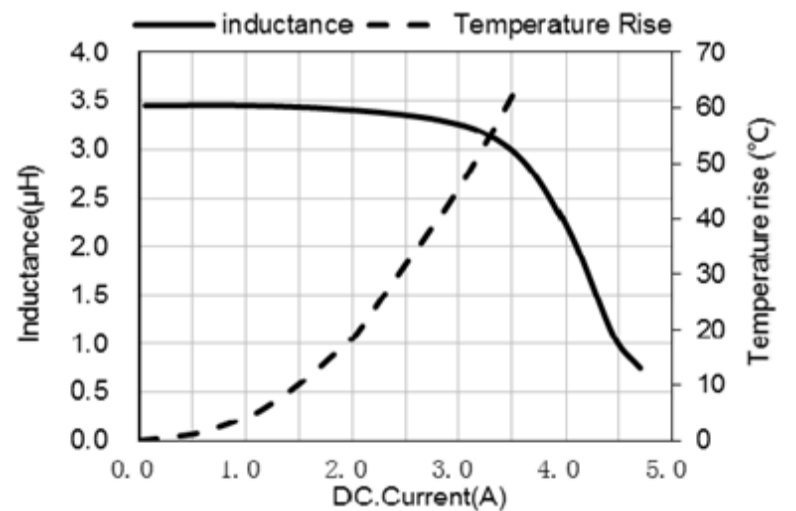
ASPIAIG-S4035-3R3
