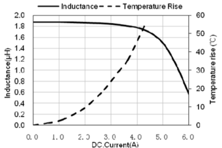
ASPIAIG-S4035-1R8
