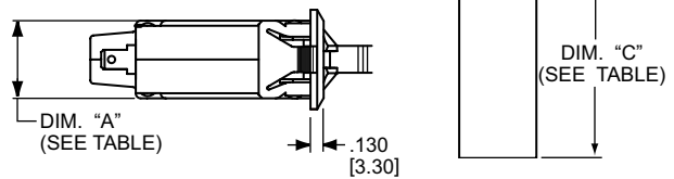
Panel Cutout Detail Panel Thickness: (See Table)
