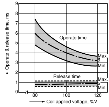
4.-(6) Operate & release time (with diode, 2 Form A)
