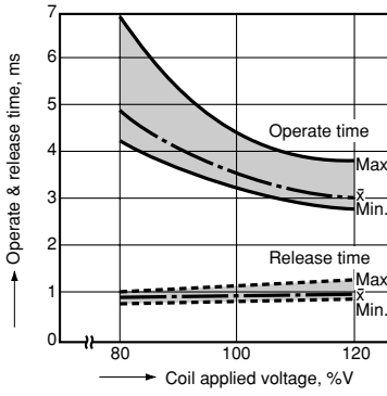
4.-(4) Operate & release time (with diode, 1 Form A)
