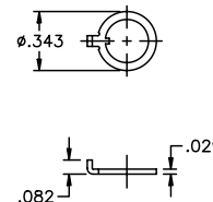
ANTI-ROTATE RING A107 Nickel plated brass 1/4
