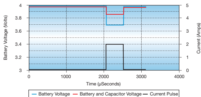
Figure 5. GSM Pulse
