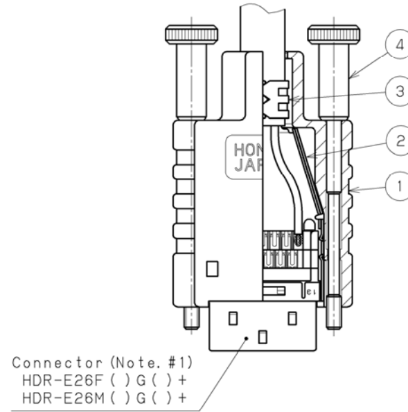
After assembly drawing
