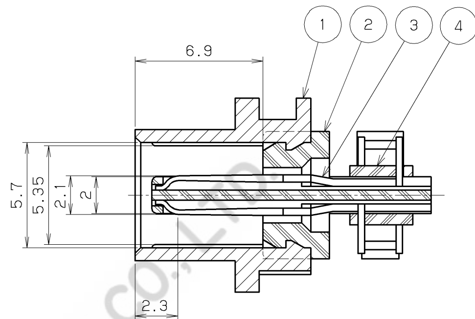
CONTACT DETAIL (5/1)
