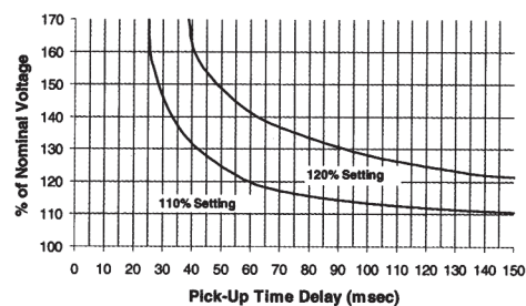
Time Curves DC Overtoltage Relays
