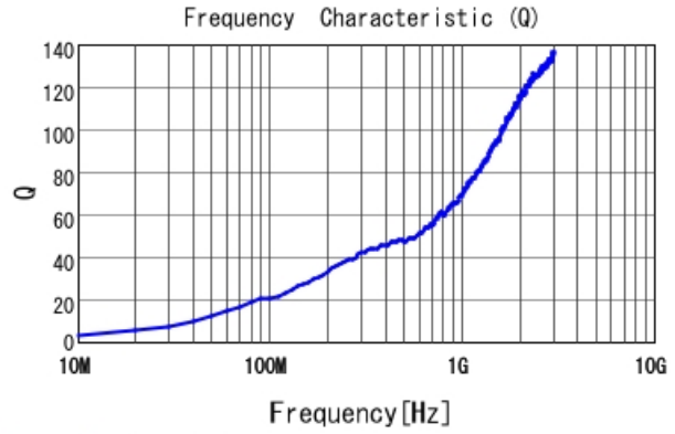
LQP15MN1N1B02 Q
