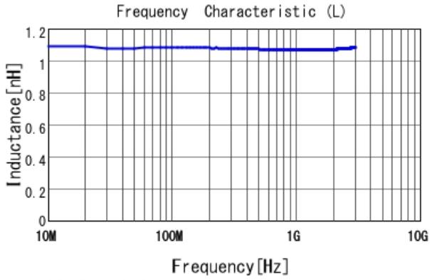
LQP15MN1N1B02 L
