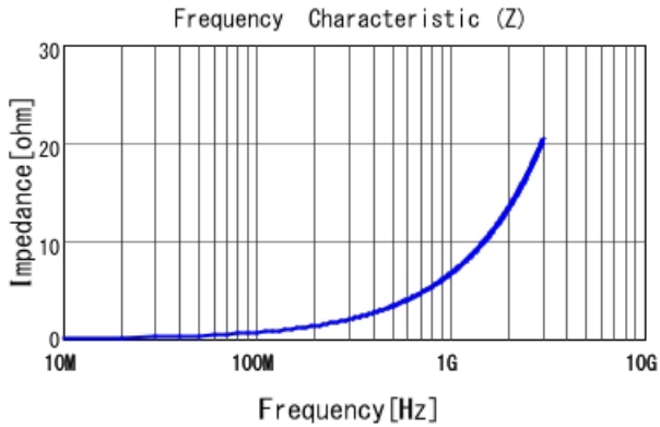
LQP15MN1N1B02 |Z|
