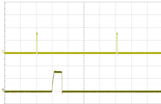
Fig. 17: Load current (top trace, 20 A/div, 100 ms/div.) into a 10 \text{ m}\Omega short circuit during restart, at V_{in} = 48 \text{ V} . Bottom trace (20 A/div., 10 ms/div.) is an expansion of the on-time portion of the top trace
