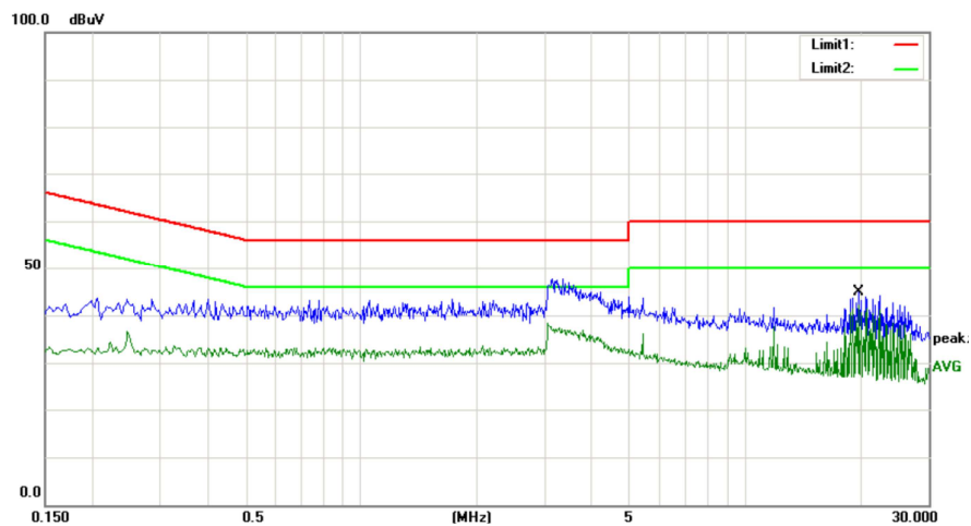
Fig. 20: Vin- Peak Detector EMI waveform
