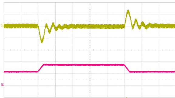
Fig. 11: Output voltage response to load current step change (12A – 18A – 12A) at V_{in} = 48\text{ V} . Top trace: output voltage (200 mV/div.). Bottom trace: load current (10 A/div.). Current slew rate: 0.1 A/ \mu\text{s} . C_o = 1\ \mu\text{F} ceramic + 10 \mu\text{F} tantalum. Time scale: 200 \mu\text{s} /div.
