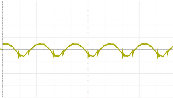
Fig. 13: Output voltage ripple (50 mV/div.) at full rated load currents, current into a resistive load with C_o = 10 \mu\text{F} tantalum + 1 \mu\text{F} ceramic and V_{in} = 48 \text{ V} . Time scale: 2 \mu\text{s}/\text{div} .
