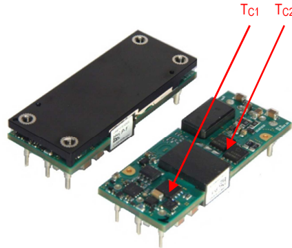
Fig. G: Locations of the thermocouples for thermal testing.
