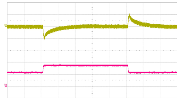
Fig. 12: Output voltage response to load current step change (12A – 18A – 12A) at V_{in} = 48\text{ V} . Top trace: output voltage (200 mV/div.). Bottom trace: load current (10 A/div.). Current slew rate: 1 A/ \mu\text{s} . C_o = 1\ \mu\text{F} ceramic + 4,700 \mu\text{F} + 10 \mu\text{F} tantalum. Time scale: 200 \mu\text{s} /div.
