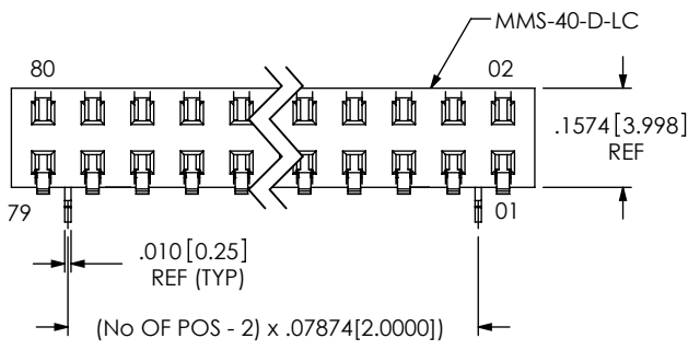
FIG 3 MMS-140-02-XXX-DH-LC SHOWN
