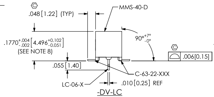
FIG 1 MMS-140-02-XXX-XV-LC SHOWN
