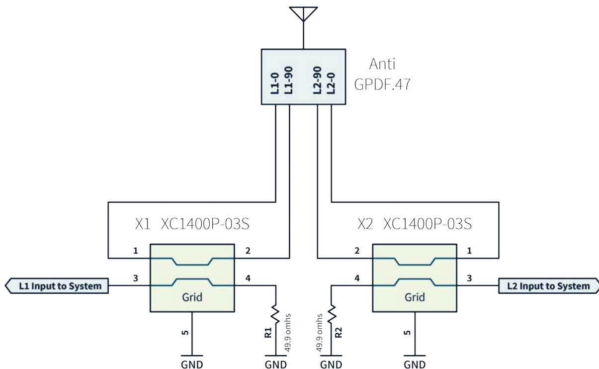
Figure 1. Schematic representation of GPDF.47.8.A.02 feed network. The pin numbers of hybrid couplers X1 and X2 follow the manufacturer's datasheet reference.
