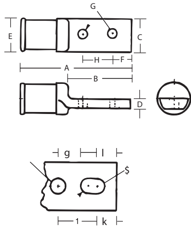
Cat. No. MD 1925 Supplied with Elongated Bolt Hole.
